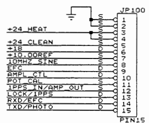
CONNECTOR TO TOP (ANALOG) PCB
